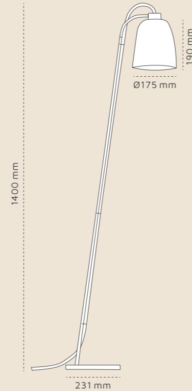
FLOOR LAMP
